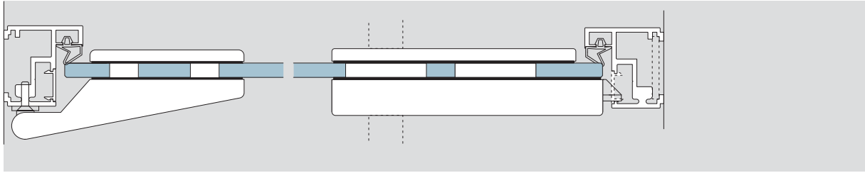
ALEXA AT 44 - with DORMA Studio (Classic, Rondo)
