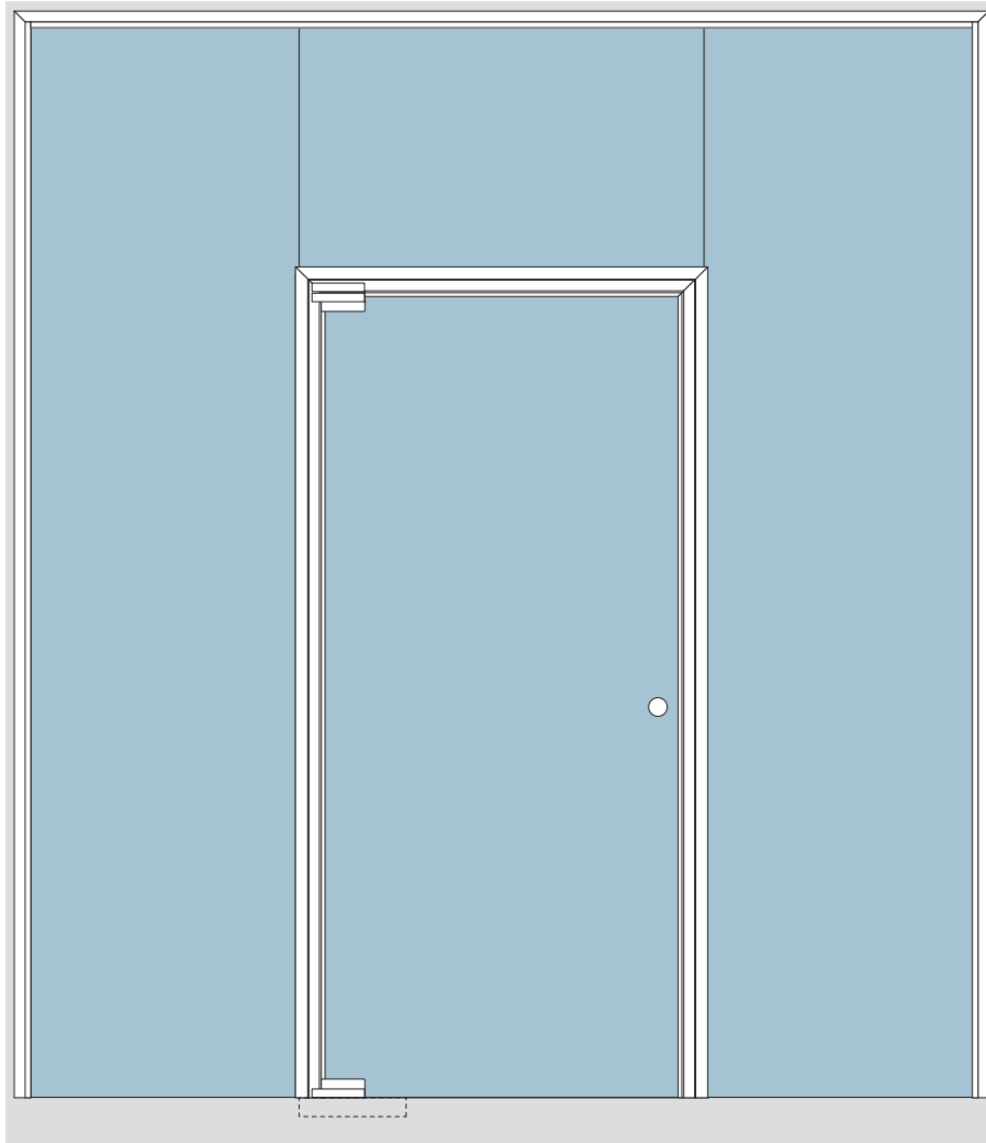
Delicate construction for fixed side lites with overpanel and centre positioned single acting door - The combination of frames ALEXA AT 44 and ALEXA PT 35.
