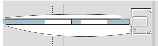
plan lock DORMA ARCOS Studio
