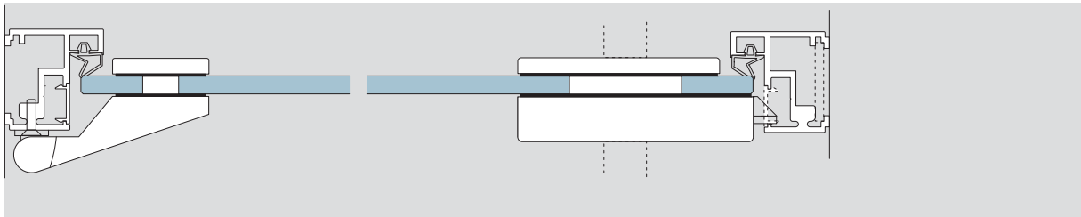
ALEXA AT 44 - with DORMA Junior (Office, Office Classic)
