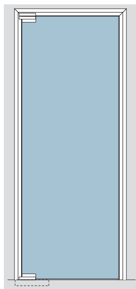
Type A ALEXA AT 44 EA 3 sided frame profile with 3 sided accessory profile for floor closer (BTS).
