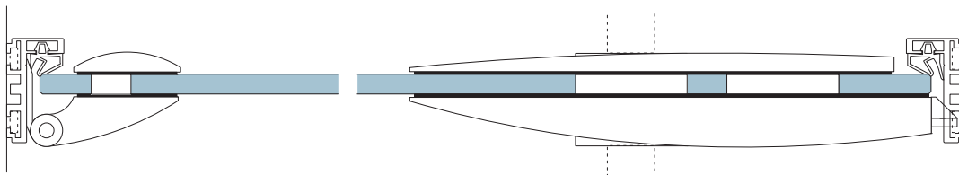
ALEXA AT 23 with DORMA special hinge ARCOS Art. no. 25.450,, lock ARCOS Studio
