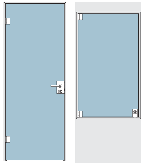
ALEXA AT 23 E Corner single acting door frame
