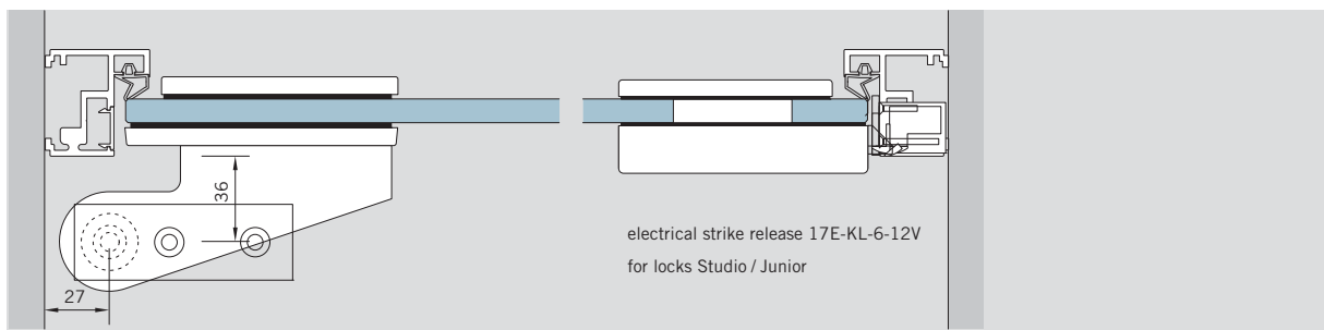
ALEXA AT 44 with DORMA EA
