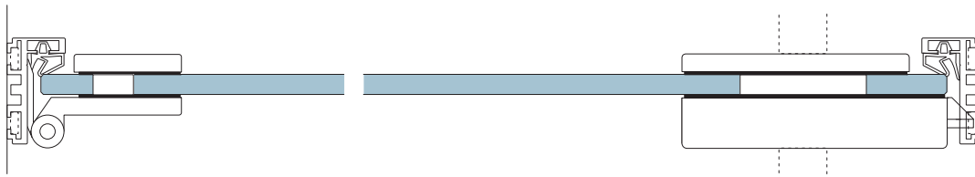
ALEXA AT 23 with DORMA special hinge Art. no. 11.294 resp. 12.050, lock Junior Office / Junior Office Classic
