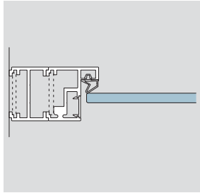
ALEXA AT 44 with accessory profile
