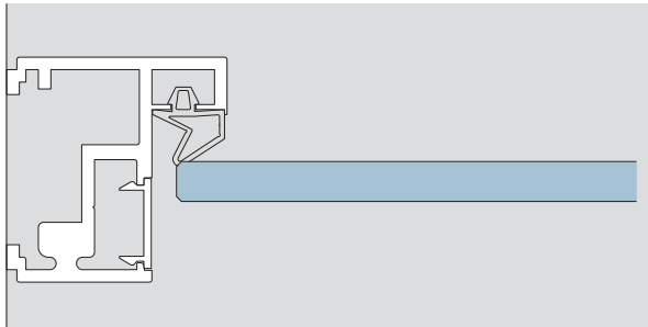
ALEXA AT 44 - frame profile
