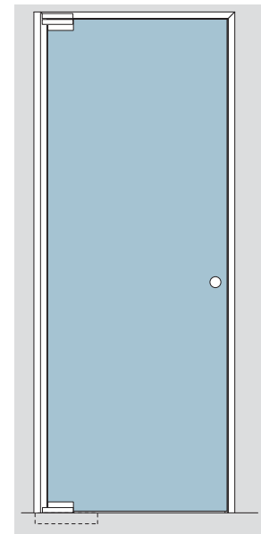
Type C ALEXA AT 44 EA 3 sided frame profile with 1 sided accessory profile for floor closer (BTS).
