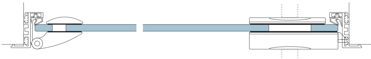
ALEXA AT 23 E with DORMA special hinge ARCOS Art. no. 25.450, lock ARCOS Office
