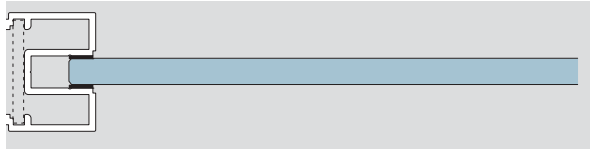
ALEXA PT 35 frame profile with glass penetration
