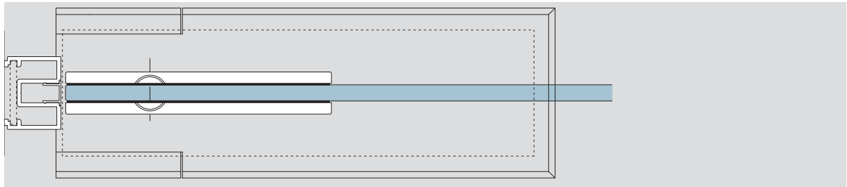
ALEXA PT 35 with DORMA Universal patch fitting, floor closer BTS 75 V
