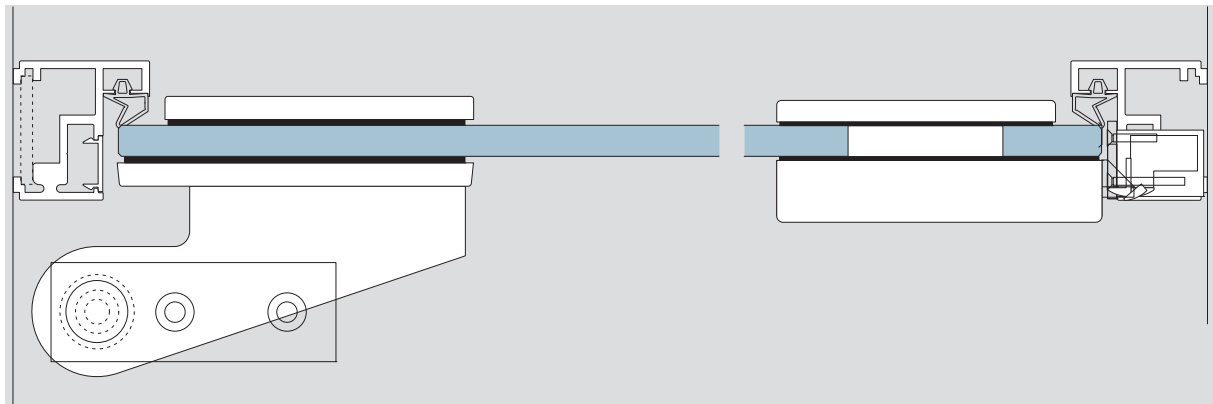
ALEXA AT 44 with DORMA EA, and floor pivot bearing Art. no. 01.106
