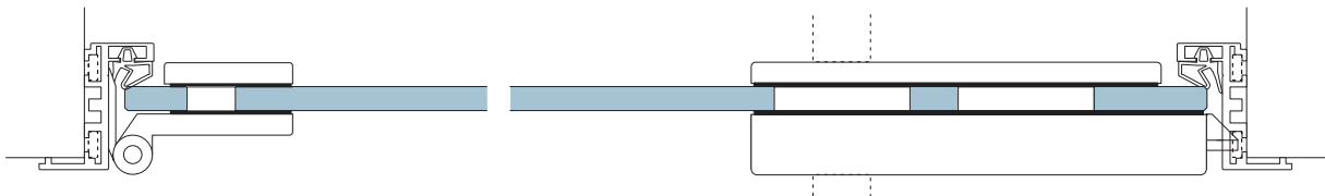
ALEXA AT 23 E with DORMA special hinge Art. no. 11.294 resp. 12.050, lock Studio Rondo / Classic
