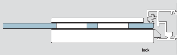
view lock Studio Rondo
