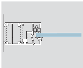
ALEXA AT 44 fixed glazing with accessory profile
