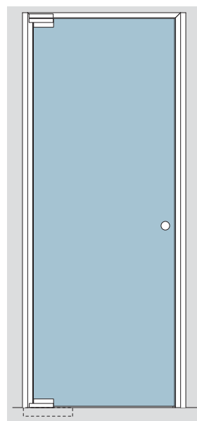
Type B ALEXA AT 44 EA 3 sided frame profile with 2 sided accessory profile for floor closer (BTS).
