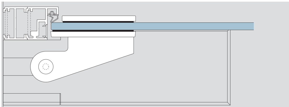
ALEXA AT 44 with DORMA EA, and floor closer DORMA BTS 75V
